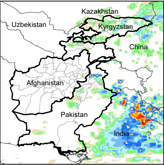
Daily Rainfall estimate for 17 Aug., 2005
