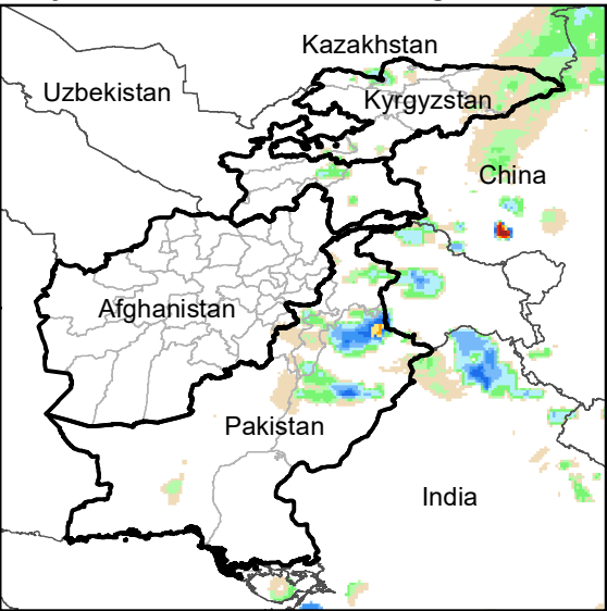
Daily Rainfall estimate for 31 Aug., 2005
