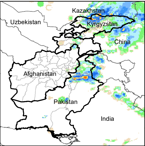
Daily Rainfall estimate for 30 Aug., 2005
