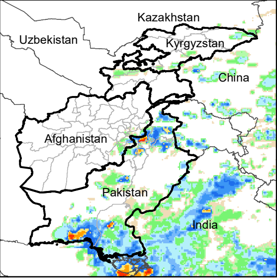
Daily Rainfall estimate for 10 Sep., 2005
