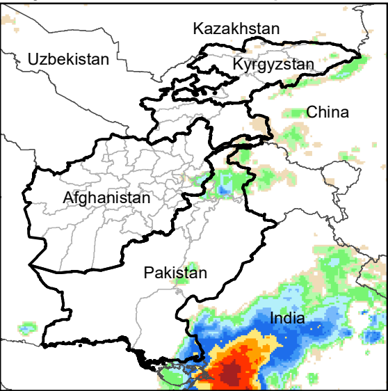
Daily Rainfall estimate for 26 Sep., 2005
