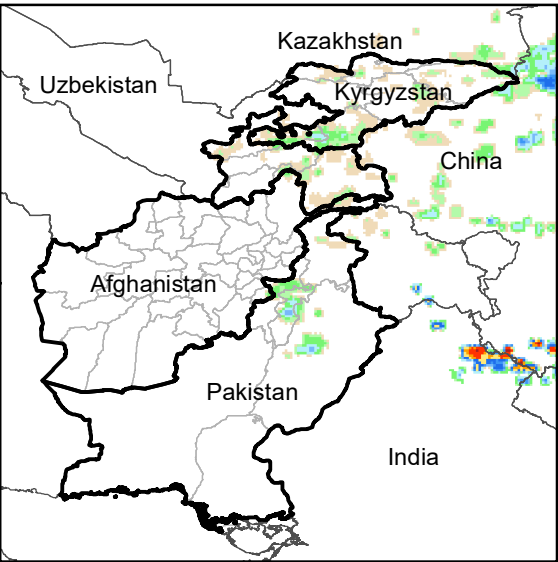
Daily Rainfall estimate for 30 Sep., 2005
