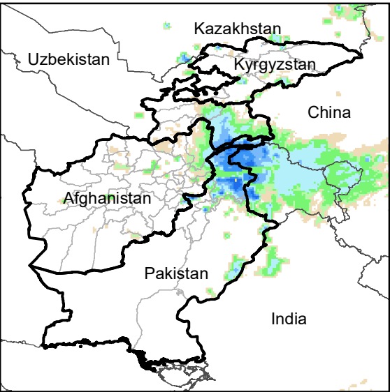
Daily Rainfall estimate for 30 Nov., 2005
