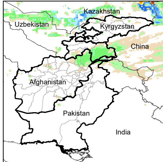
Daily Rainfall estimate for 29 Dec., 2005
