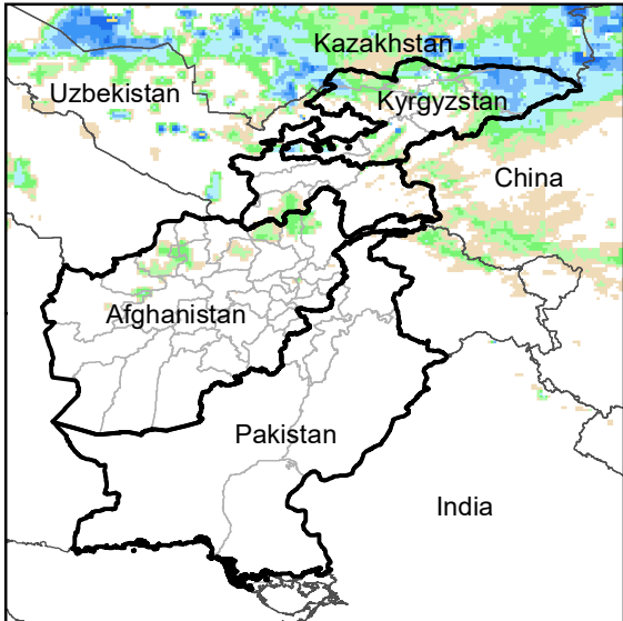
Daily Rainfall estimate for 28 Dec., 2005
