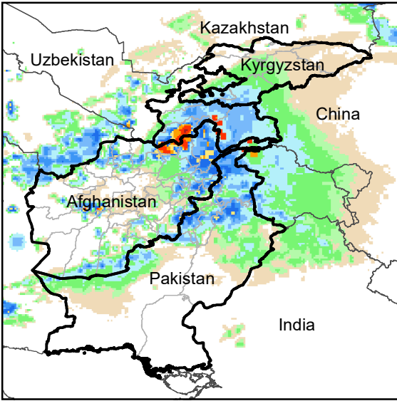
Daily Rainfall estimate for 15 Jan., 2006
