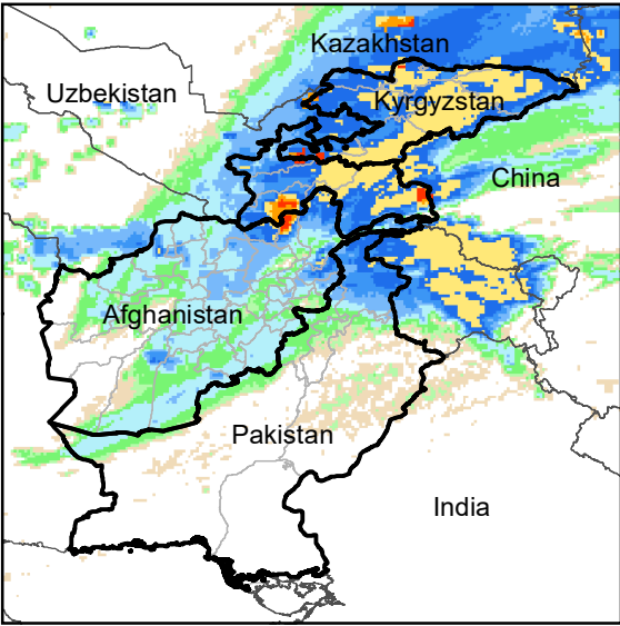
Daily Rainfall estimate for 31 Jan., 2006
