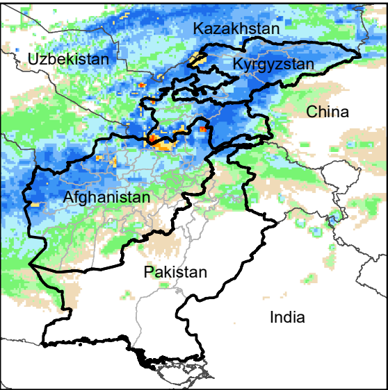
Daily Rainfall estimate for 30 Jan., 2006
