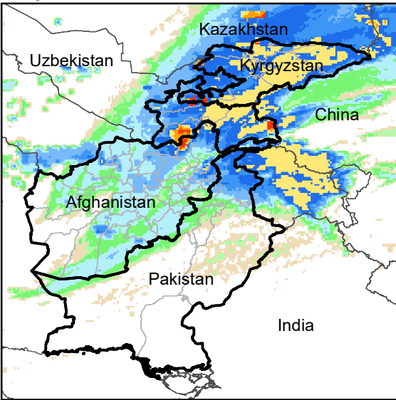
Daily Rainfall estimate for 3 Feb., 2006
