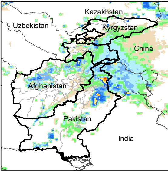
Daily Rainfall estimate for 25 Feb., 2006
