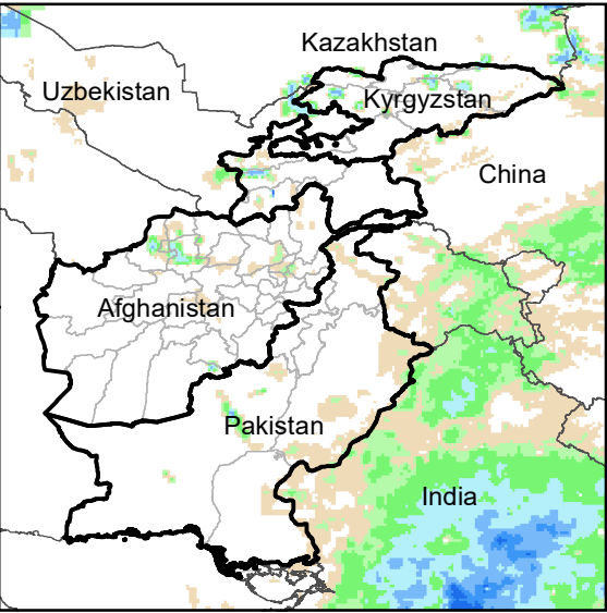
Daily Rainfall estimate for 9 Mar., 2006
