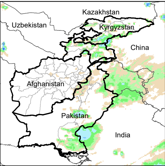
Daily Rainfall estimate for 19 Apr., 2006
