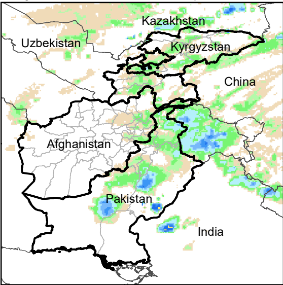
Daily Rainfall estimate for 3 May., 2006
