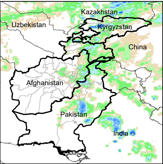
Daily Rainfall estimate for 4 May., 2006
