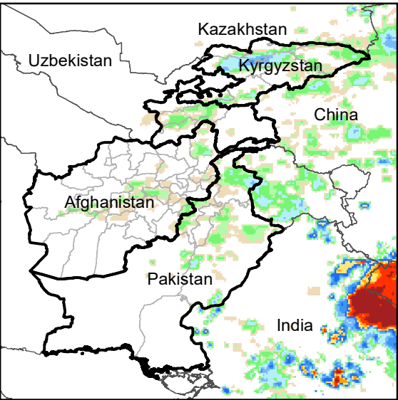
Daily Rainfall estimate for 6 Jun., 2006
