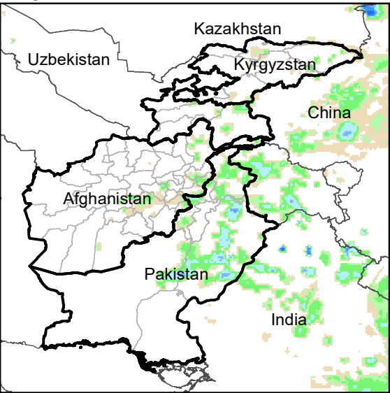
Daily Rainfall estimate for 7 Jun., 2006
