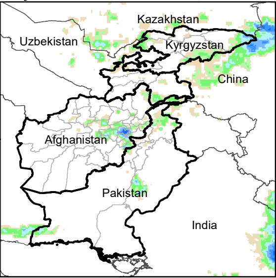
Daily Rainfall estimate for 8 Jun., 2006
