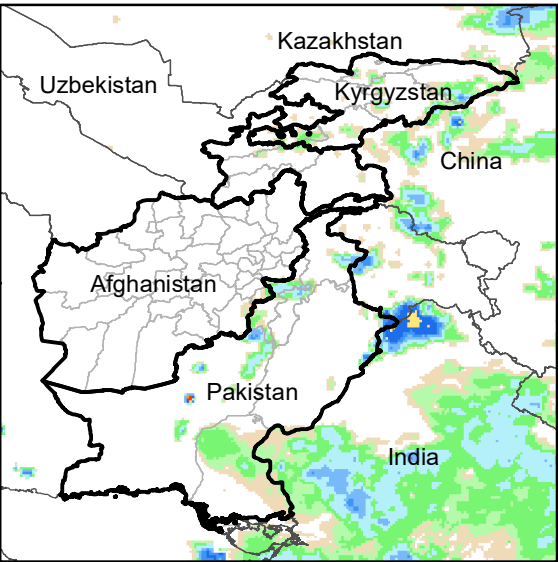
Daily Rainfall estimate for 28 Jun., 2006
