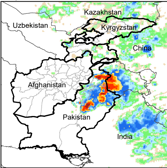
Daily Rainfall estimate for 15 Jul., 2006
