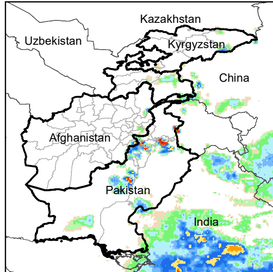
Daily Rainfall estimate for 21 Jul., 2006
