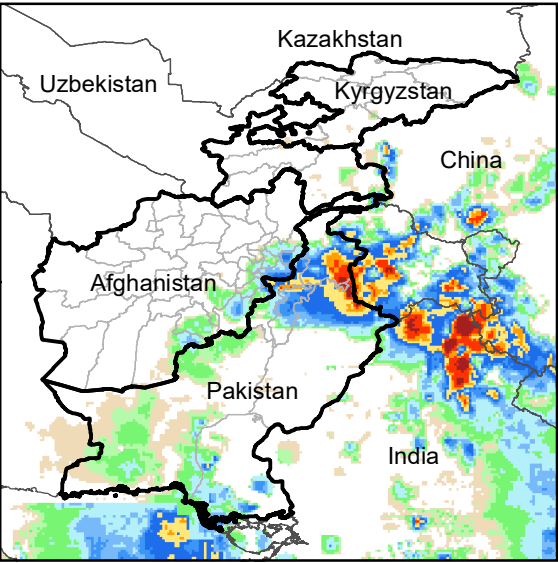
Daily Rainfall estimate for 2 Aug., 2006
