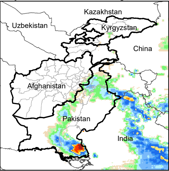
Daily Rainfall estimate for 23 Aug., 2006
