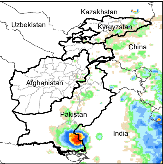
Daily Rainfall estimate for 25 Aug., 2006
