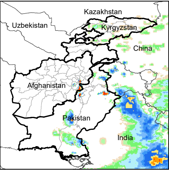
Daily Rainfall estimate for 24 Aug., 2006
