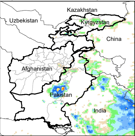
Daily Rainfall estimate for 28 Aug., 2006
