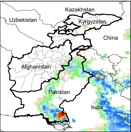
Daily Rainfall estimate for 26 Aug., 2006
