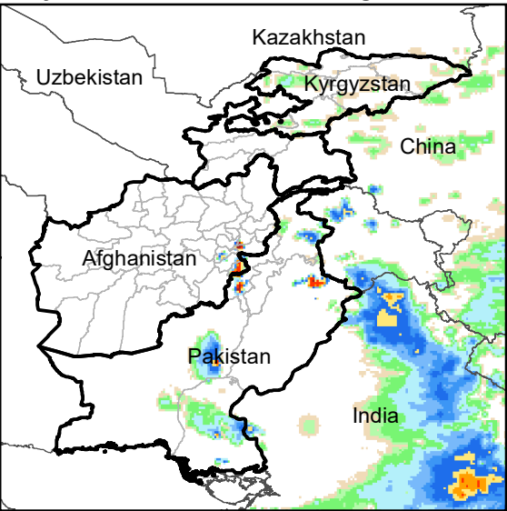
Daily Rainfall estimate for 27 Aug., 2006
