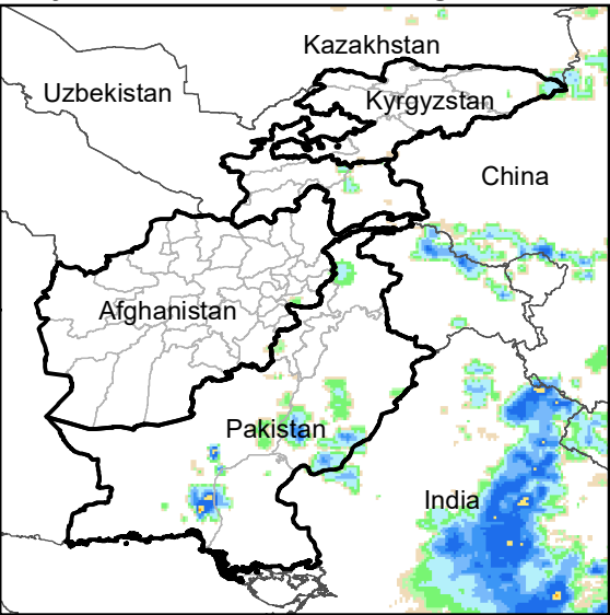
Daily Rainfall estimate for 2 Sep., 2006
