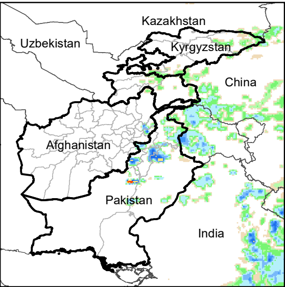
Daily Rainfall estimate for 1 Sep., 2006
