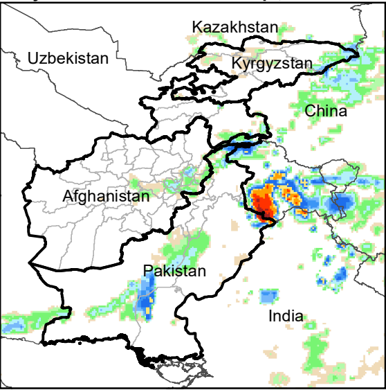
Daily Rainfall estimate for 3 Sep., 2006
