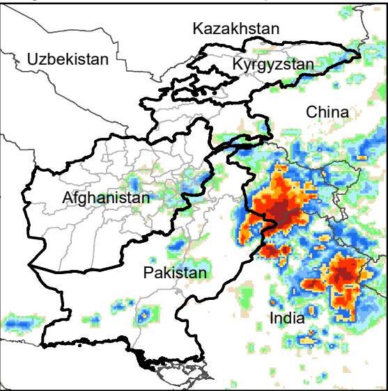
Daily Rainfall estimate for 5 Sep., 2006
