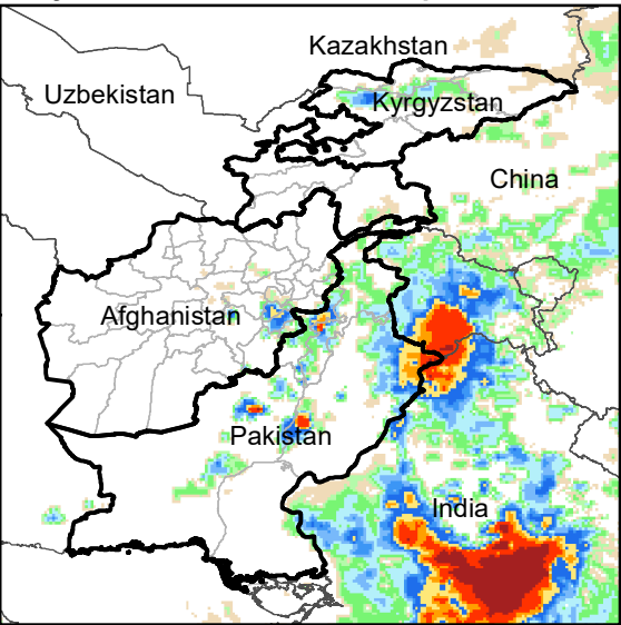
Daily Rainfall estimate for 4 Sep., 2006
