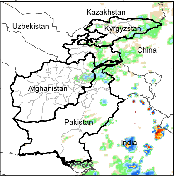
Daily Rainfall estimate for 21 Sep., 2006
