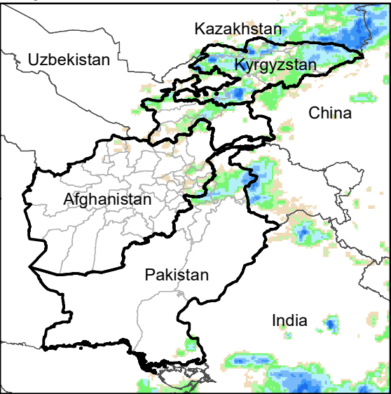
Daily Rainfall estimate for 22 Sep., 2006
