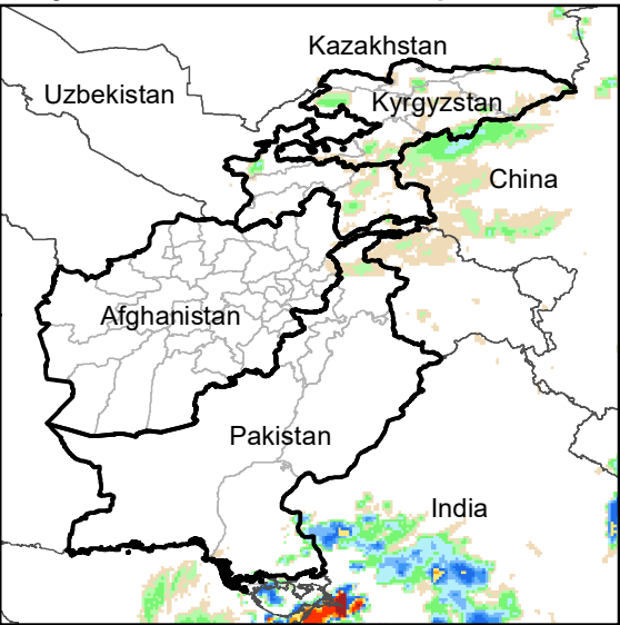
Daily Rainfall estimate for 27 Sep., 2006
