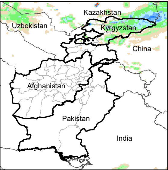
Daily Rainfall estimate for 7 Oct., 2006
