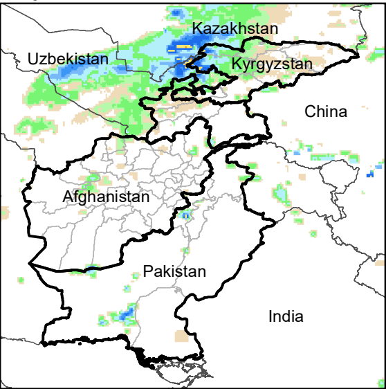
Daily Rainfall estimate for 1 Nov., 2006
