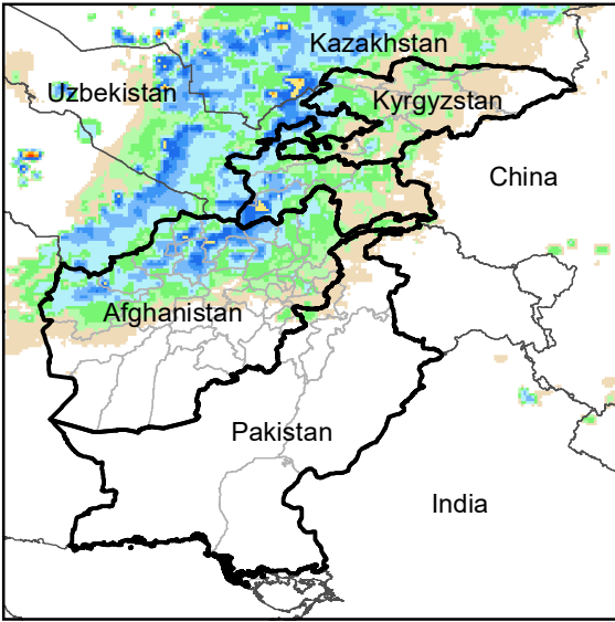
Daily Rainfall estimate for 9 Nov., 2006
