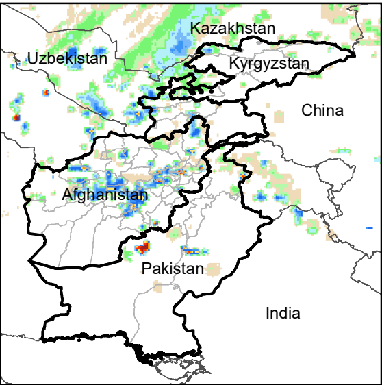
Daily Rainfall estimate for 22 Nov., 2006
