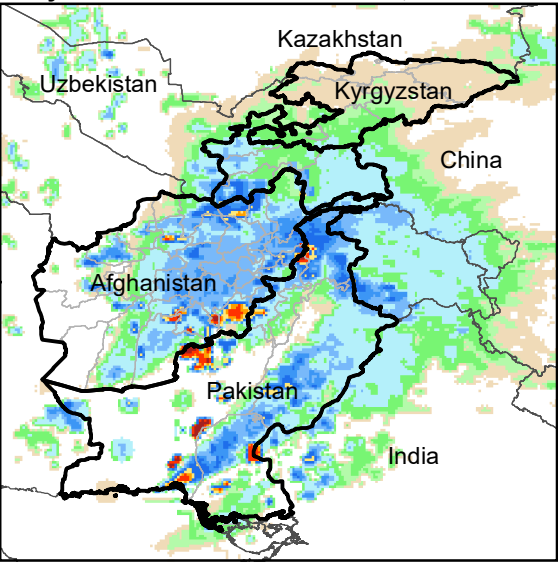
Daily Rainfall estimate for 4 Dec., 2006
