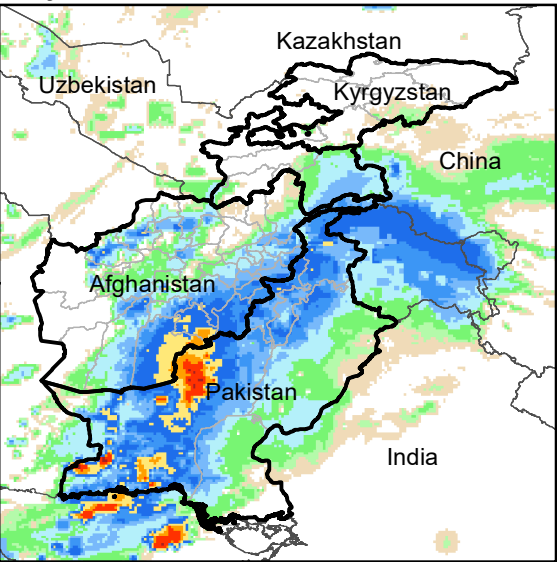
Daily Rainfall estimate for 6 Dec., 2006
