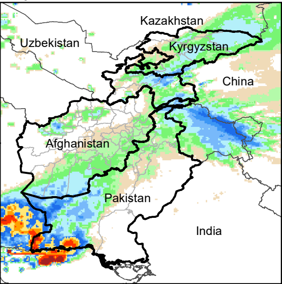
Daily Rainfall estimate for 5 Dec., 2006
