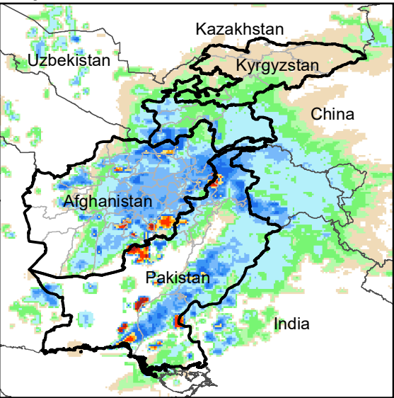
Daily Rainfall estimate for 7 Dec., 2006
