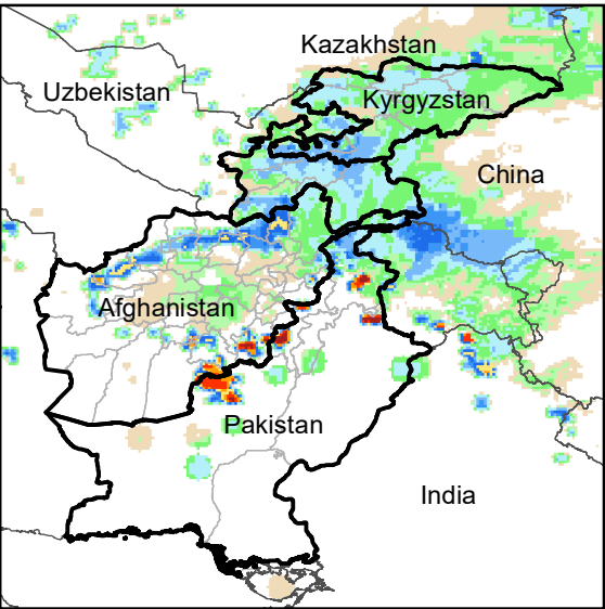
Daily Rainfall estimate for 8 Dec., 2006
