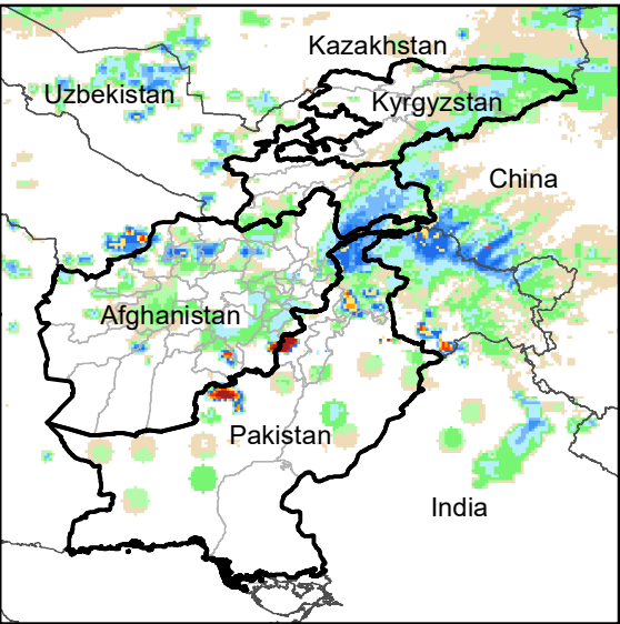
Daily Rainfall estimate for 29 Dec., 2006
