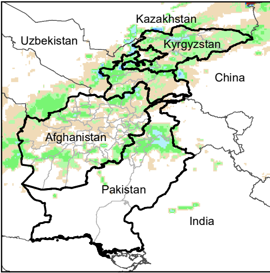
Daily Rainfall estimate for 3 Feb., 2007
