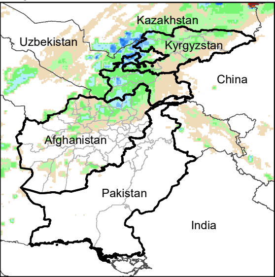
Daily Rainfall estimate for 5 Feb., 2007
