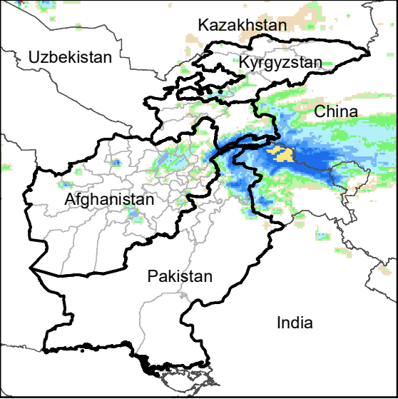
Daily Rainfall estimate for 4 Mar., 2007
