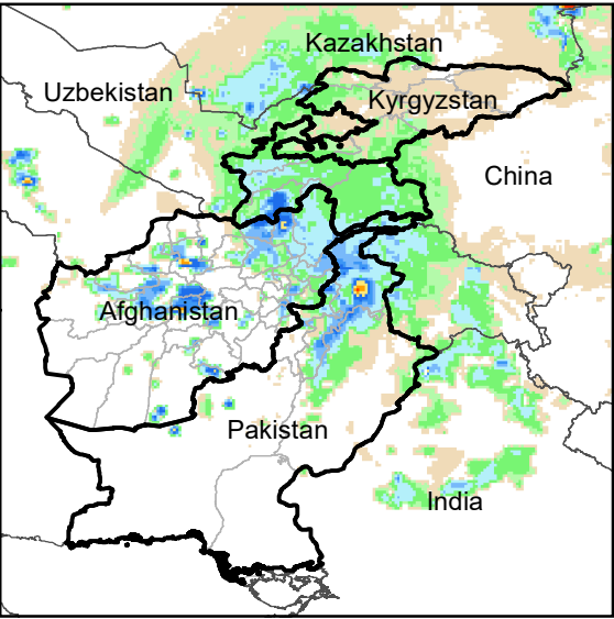
Daily Rainfall estimate for 9 Mar., 2007
