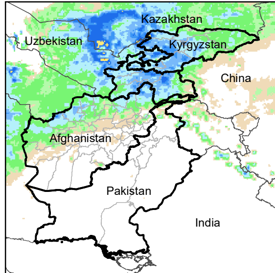
Daily Rainfall estimate for 28 Mar., 2007
