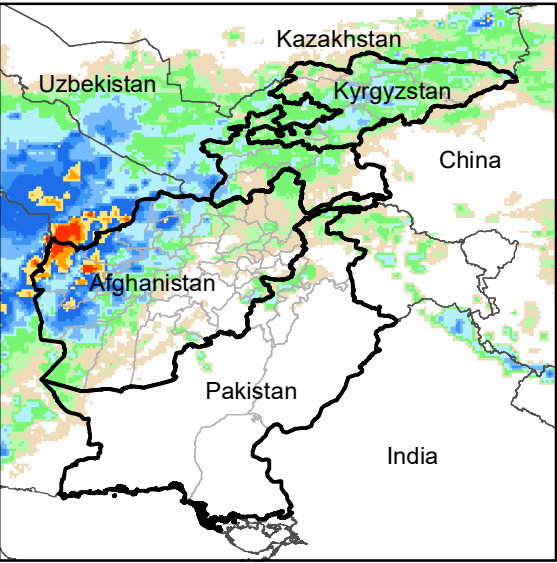
Daily Rainfall estimate for 29 Mar., 2007
