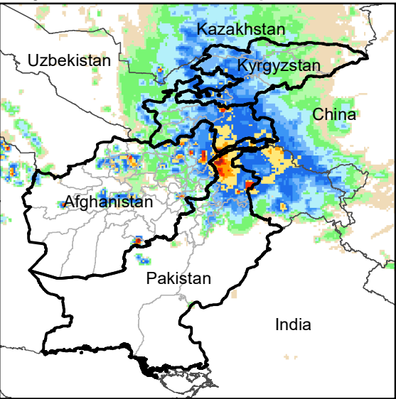
Daily Rainfall estimate for 4 Apr., 2007
