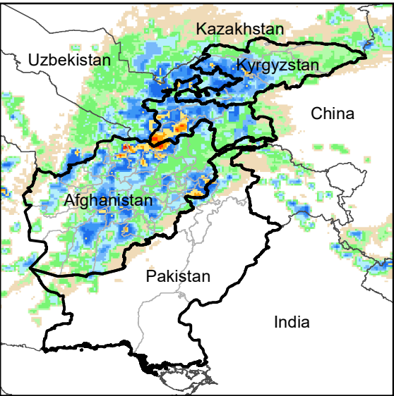
Daily Rainfall estimate for 2 Apr., 2007
