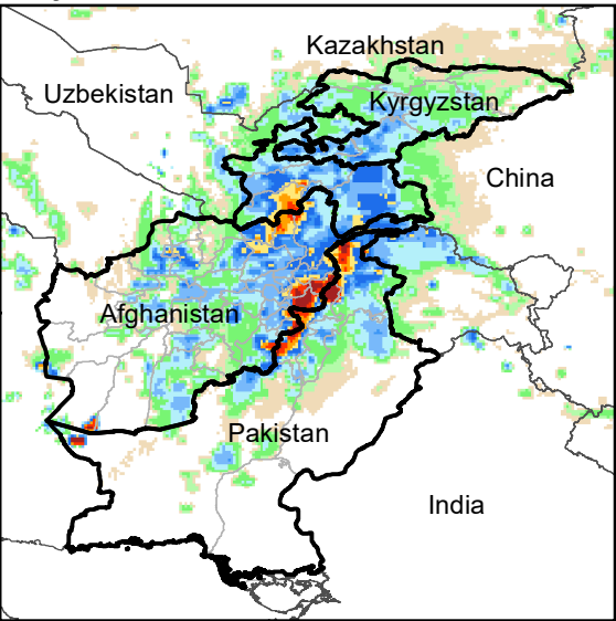
Daily Rainfall estimate for 3 Apr., 2007
