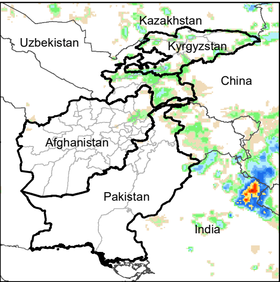
Daily Rainfall estimate for 12 May., 2007
