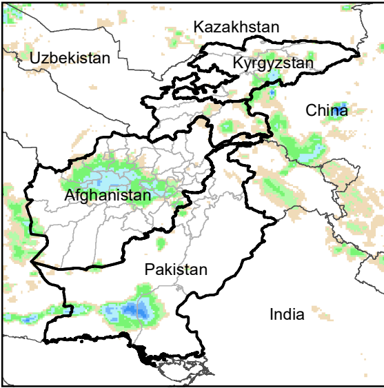
Daily Rainfall estimate for 14 May., 2007
