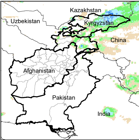
Daily Rainfall estimate for 16 May., 2007
