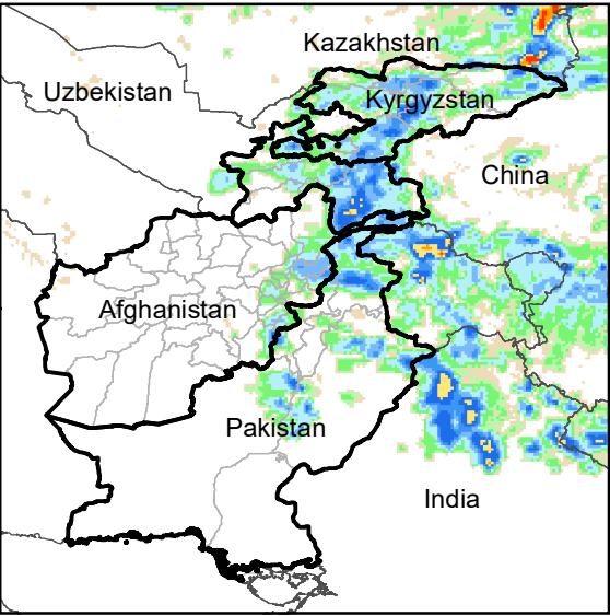
Daily Rainfall estimate for 26 May., 2007
