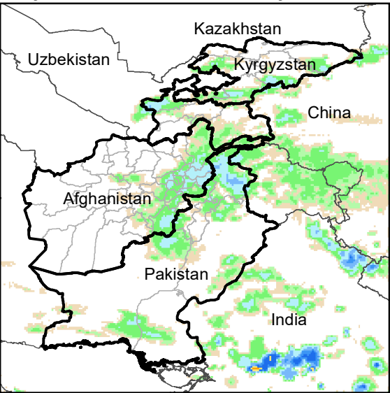
Daily Rainfall estimate for 1 Jun., 2007
