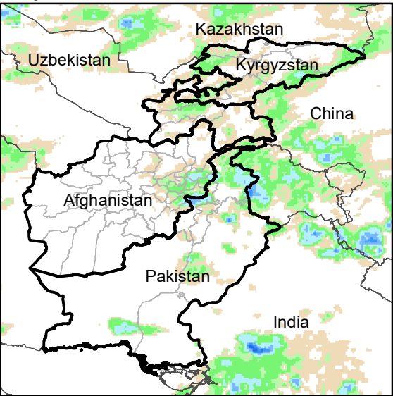
Daily Rainfall estimate for 6 Jun., 2007
