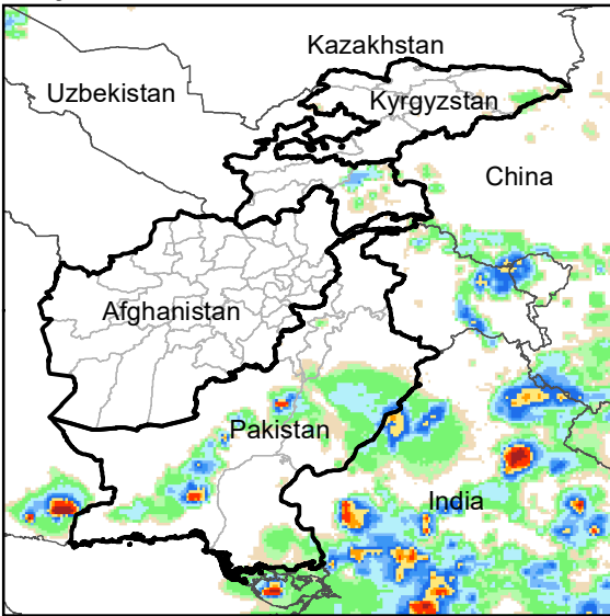
Daily Rainfall estimate for 23 Jun., 2007
