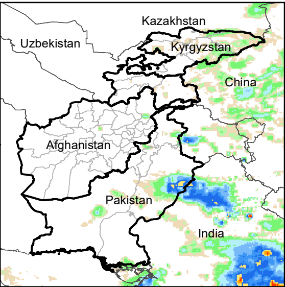
Daily Rainfall estimate for 21 Jun., 2007
