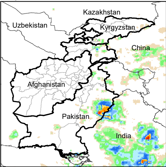
Daily Rainfall estimate for 22 Jun., 2007
