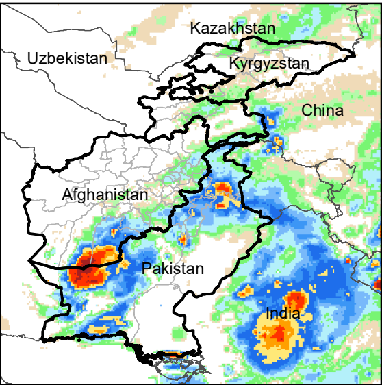
Daily Rainfall estimate for 1 Jul., 2007
