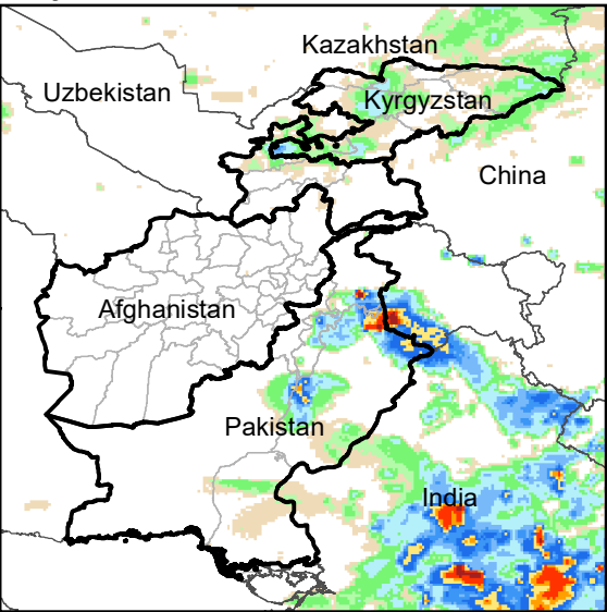
Daily Rainfall estimate for 9 Jul., 2007
