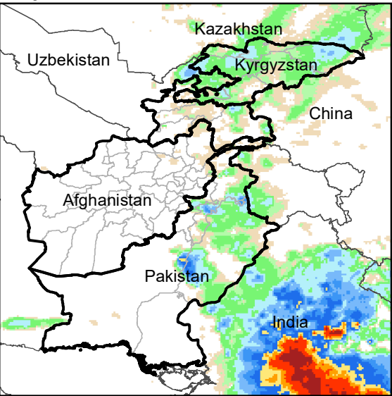
Daily Rainfall estimate for 10 Jul., 2007
